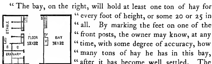
Fig. 14.—Principal Floor.
